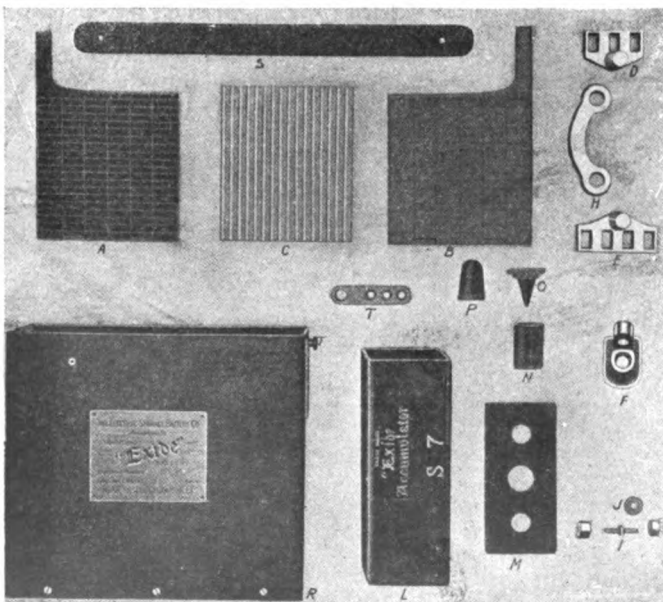
Complete Set of Parts of Sparking Battery Dissembled.
